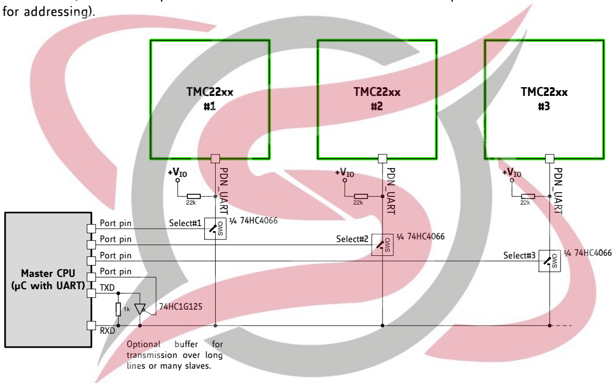
Figure 4.2 Addressing multiple TMC2209 via single wire interface using analog switches
