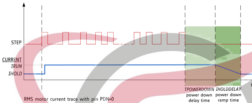
Figure 1.4 Automatic Motor Current Power Down
