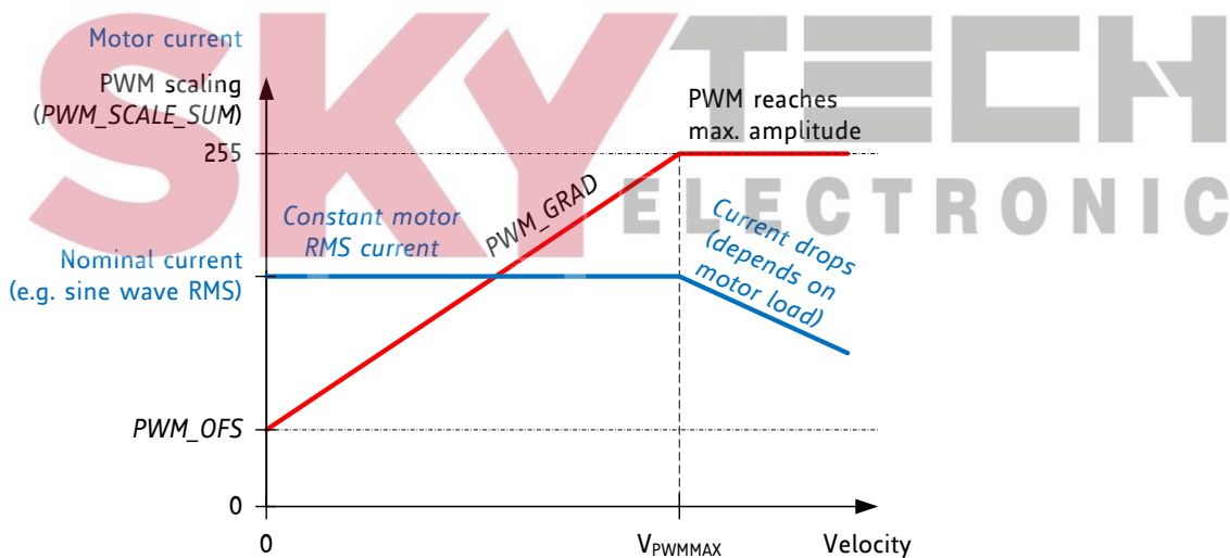
Figure 6.6 Velocity based PWM scaling (pwm_autoscale=0)
