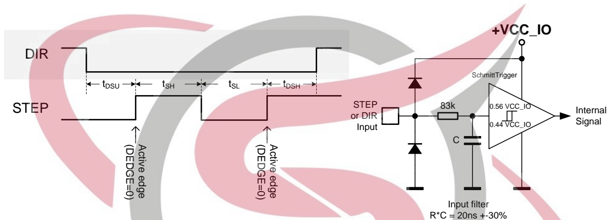
Figure 13.1 STEP and DIR timing, Input pin filter
