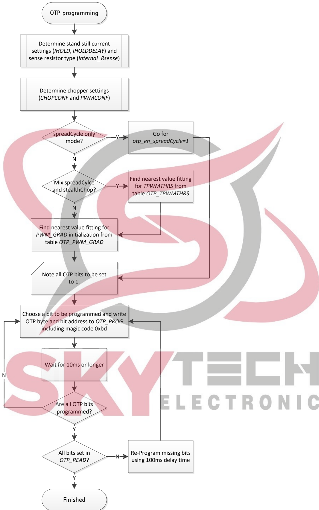
Figure 16.4 OTP programming
