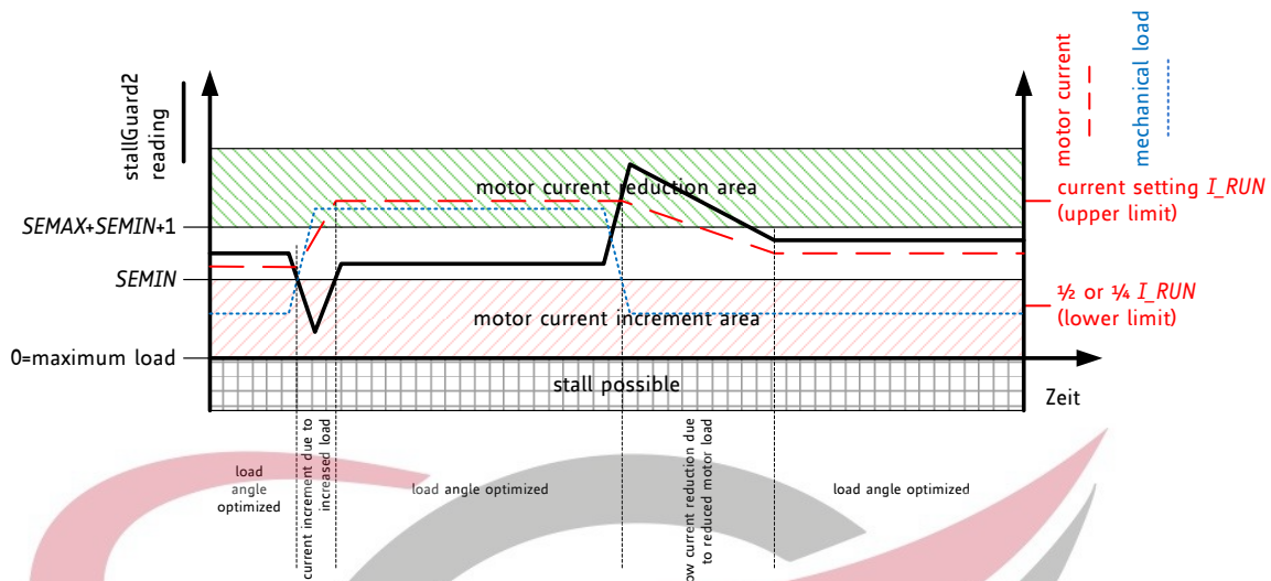
Figure 12.1 CoolStep adapts motor current to the load
